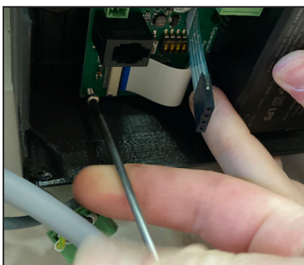
26. Secure the control unit in the right place with the six screws.
